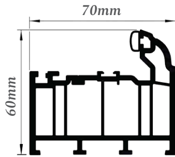
Outer Frame
